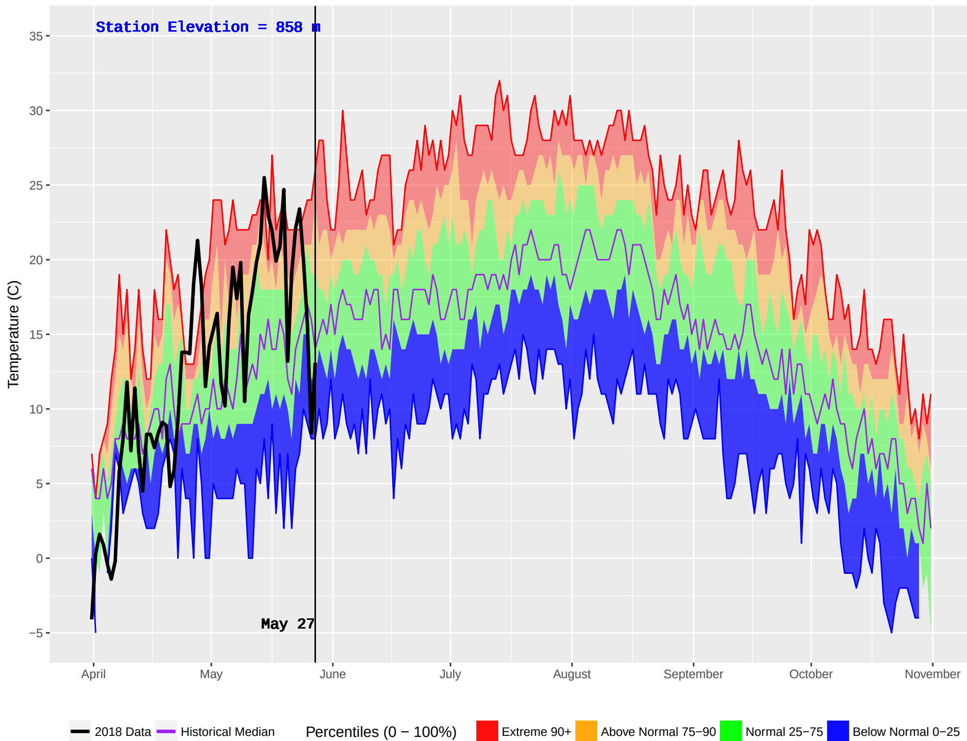
BEDNESTI (175) : Historical (1993–2016) and Current (2018) Noon Temperature
