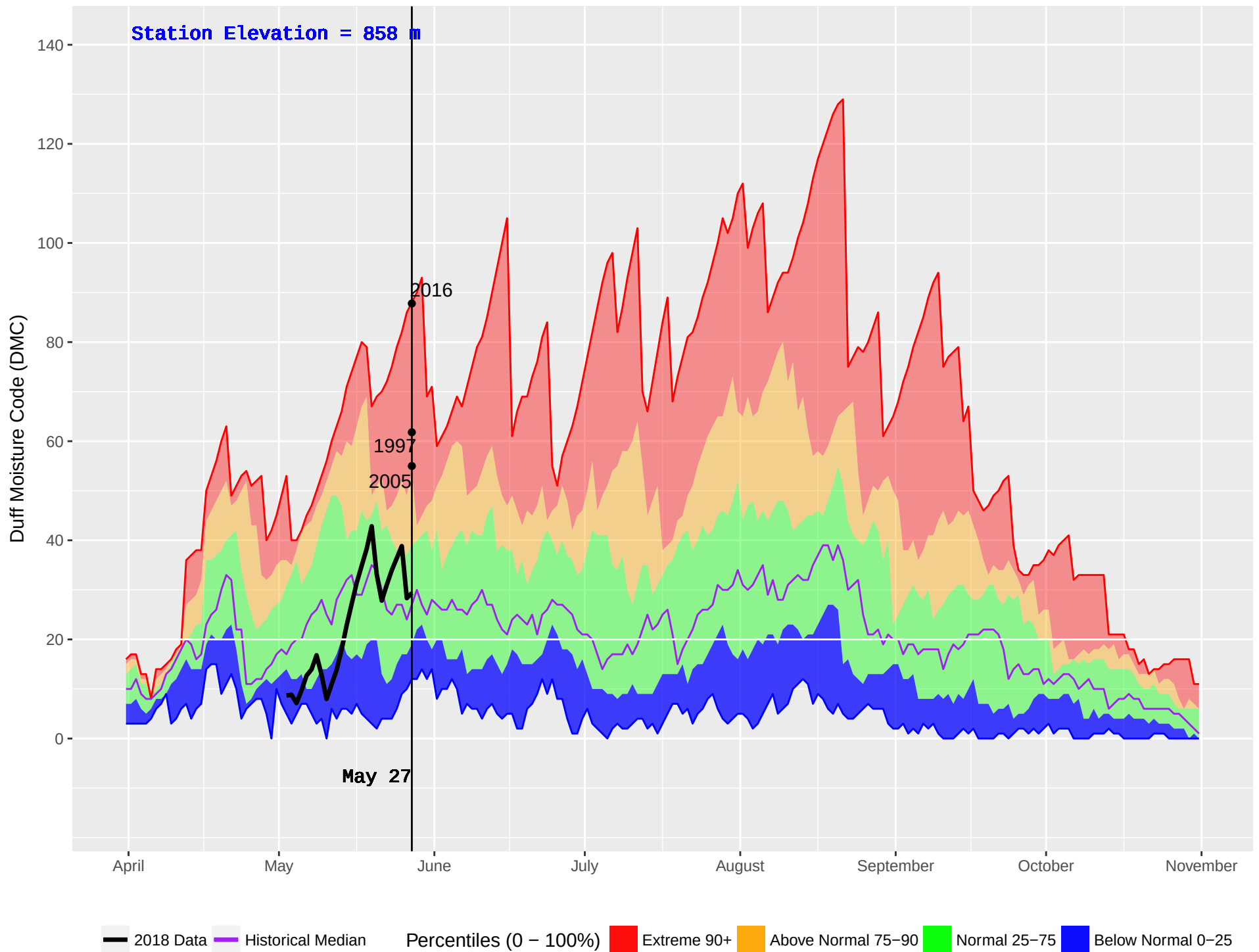
BEDNESTI (175) : Historical (1993–2016) and Current (2018) Noon Duff Moisture Code (DMC)
