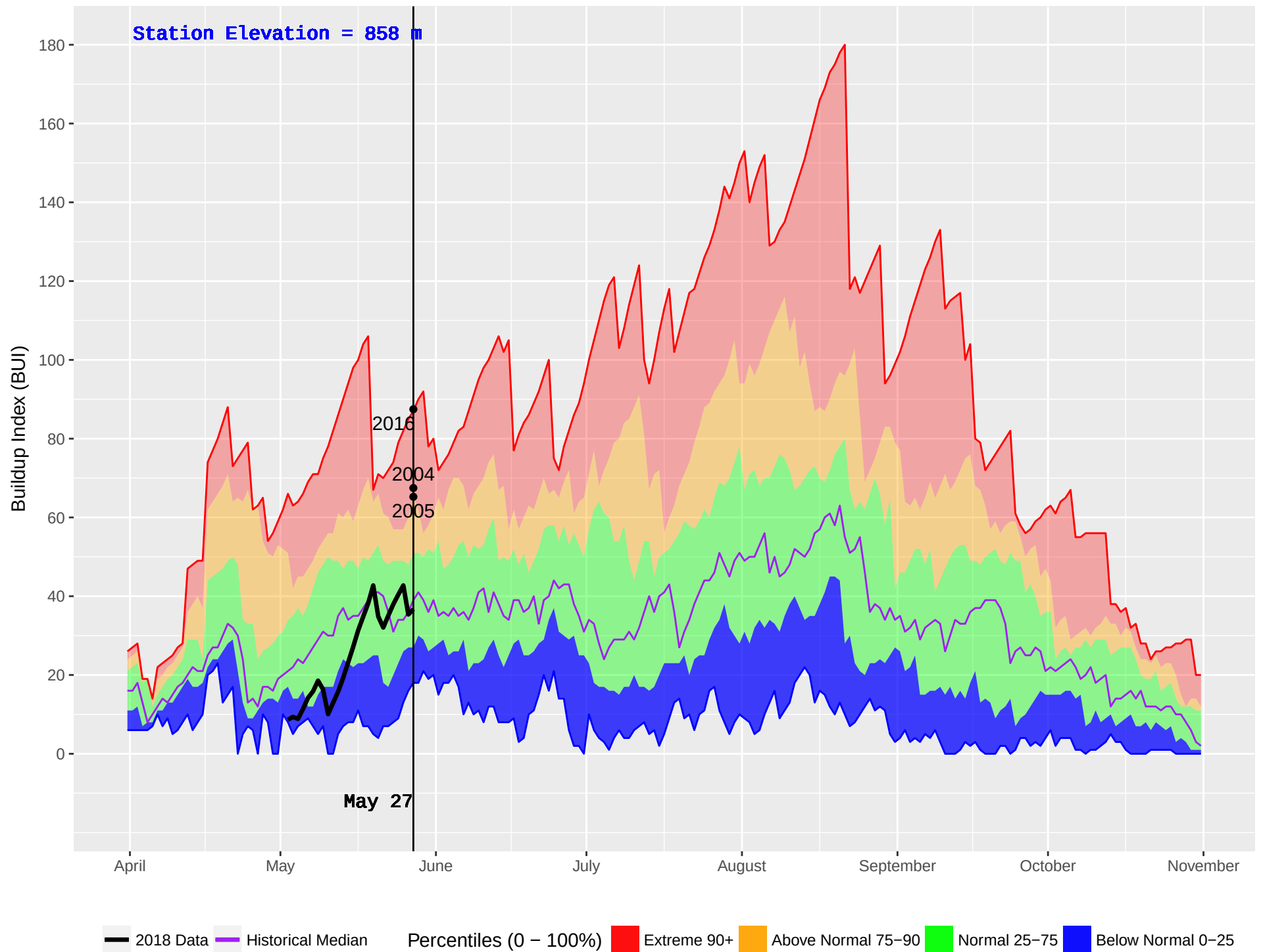
BEDNESTI (175) : Historical (1993–2016) and Current (2018) Noon Buildup Index (BUI)
