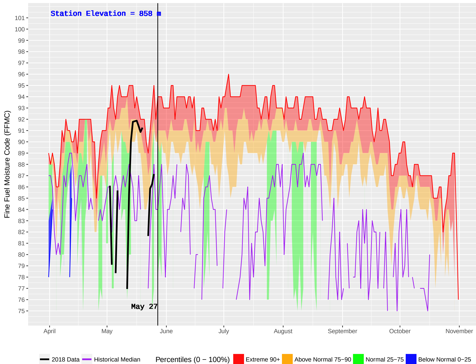
BEDNESTI (175) : Historical (1993–2016) and Current (2018) Noon Fine Fuel Moisture Code (FFMC)
